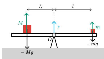
Figure 2.66: Free-body diagram of the seesaw and the masses.
