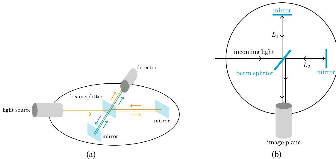
Figure 3.196: Michelson & Morley setup
