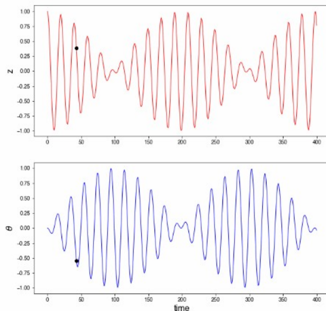
Figure 2.129: Animation of the Wilberforce pendulum using a higher-order numerical method.
