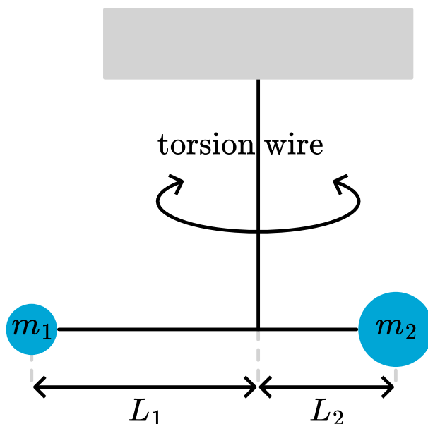
Figure 2.31: Torsion balance used by Eötvös.
