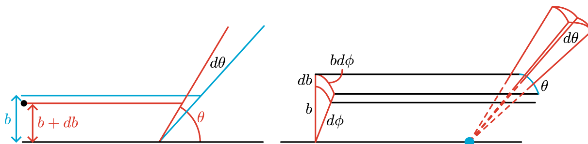
Figure 3.193: left: scattering in 2D, right: scattering in 3D.
