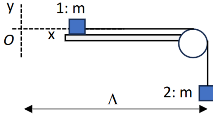
Figure 4.241: The x and y axes are represented as dotted lines. The origin of the coordinate system is O.
