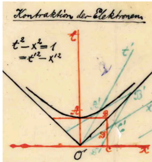
Figure 3.231: Drawing by Minkowski
