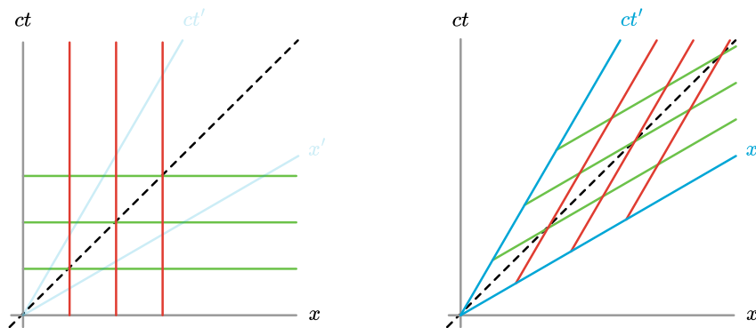
Figure 3.220: Left: lines of equal time (green) and equal space coordinate (red) in frame of reference S (left) and S' (right). For the frame of reference S' that is a bit different.
