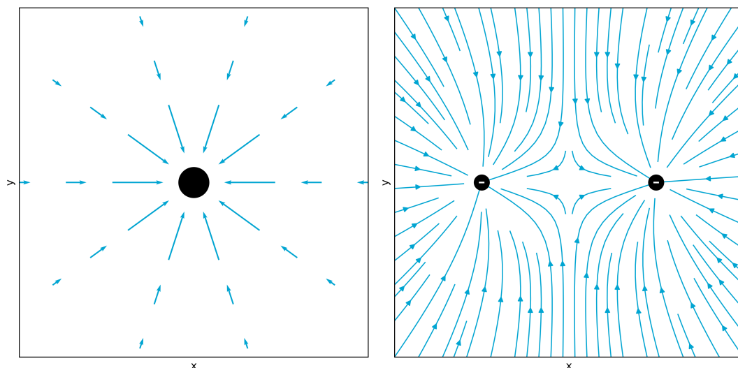
Figure 2.28: The force field that a positively charged particle would feel due to the presence of 2 negatively charged particles (both of the same charge).
