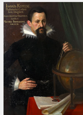
Figure 2.81: Johannes Kepler (1571-1630).
