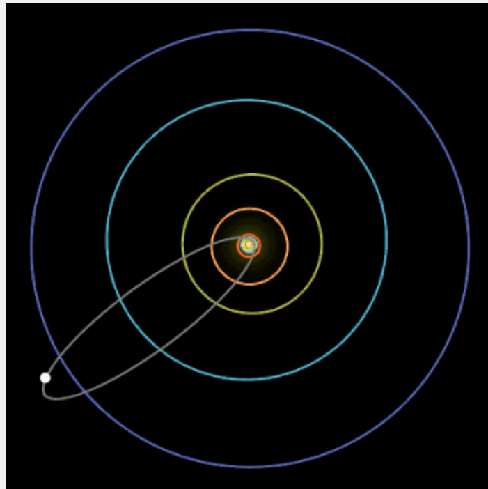
Figure 2.92: Trajectory of Haley's comet. From Wikimedia Commons , licensed under CC-BY 4.0.
