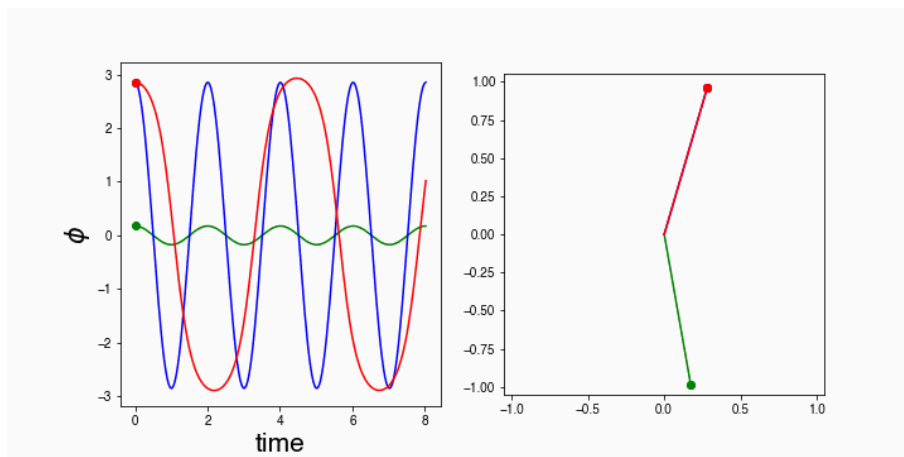
Figure 2.138: Animation of the pendulum: red is the true pendulum, blue the small angle approximation applied to a large angle case and green the small angle approximation for a small angle.
