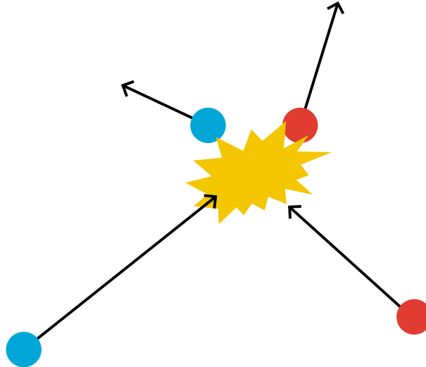
Figure 2.155: Collision of two particles.
