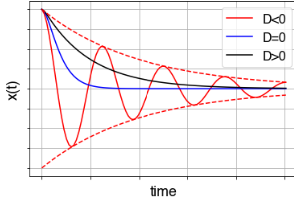
Figure 2.139: Different cases for the damped harmonic oscillator.
