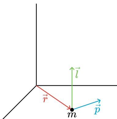
Figure 2.70: Angular momentum of a particle at a certain position with momentum.
