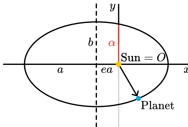
Figure 2.89: Ellipse in Cartesian coordinates.
