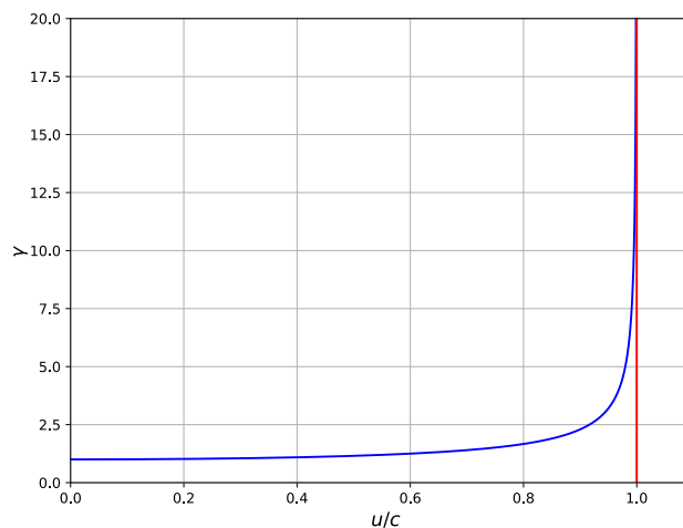
Figure 3.235: The \gamma factor increases strongly if the speed approaches the speed of light u/c \rightarrow 1
