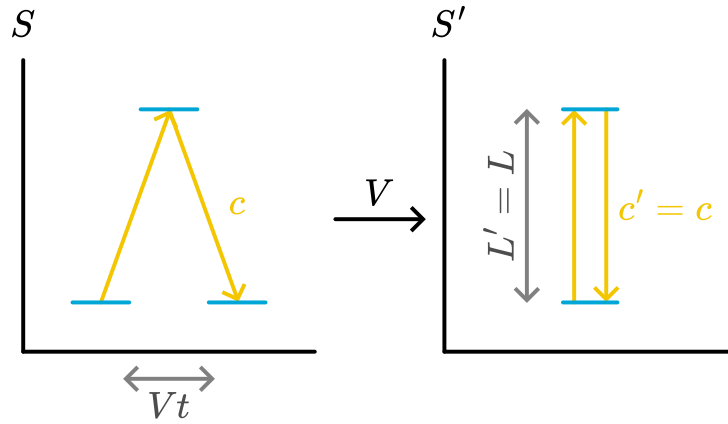
Figure 3.201: Clock stationary according to S' but moving for S .
