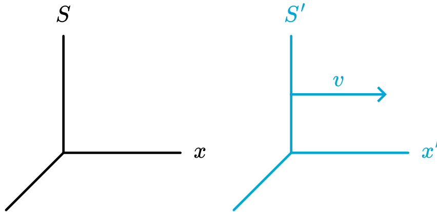
Figure 3.198: S and S' : relative velocity parallel to the x and x' axes.
