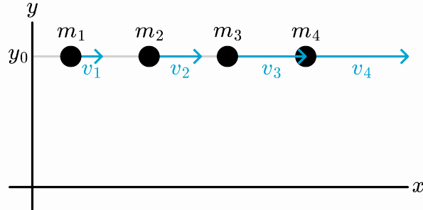
Figure 2.182: Four particles moving on a line.
