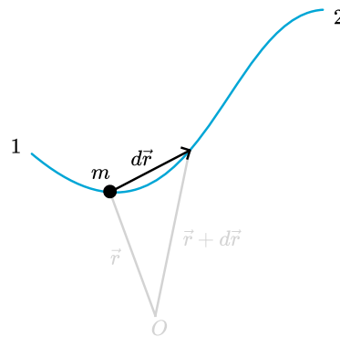
Figure 2.51: Path of a particle.
