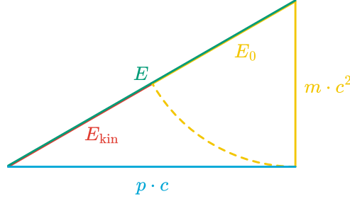
Figure 3.234: Einstein triangle.
