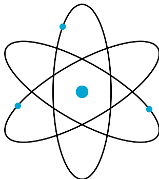
Figure 3.190: Rutherford's model of an atom.
