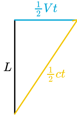
Figure 3.202: Light path in a moving clock.
