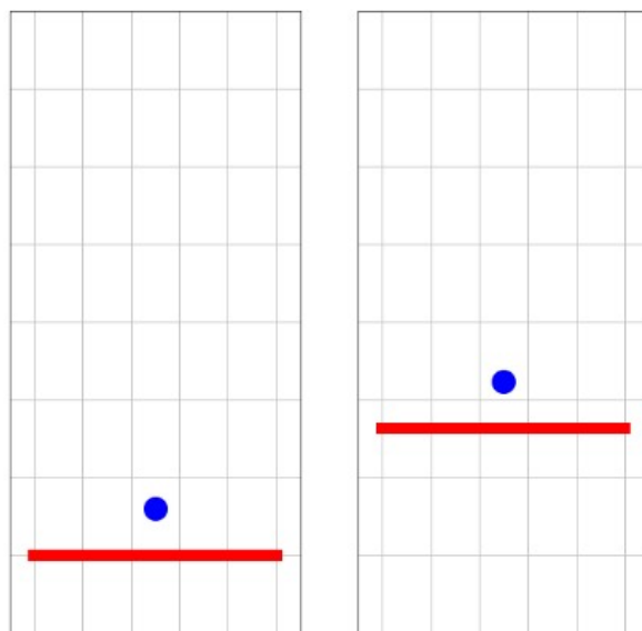
Figure 2.116: Ball bouncing at a wall.
