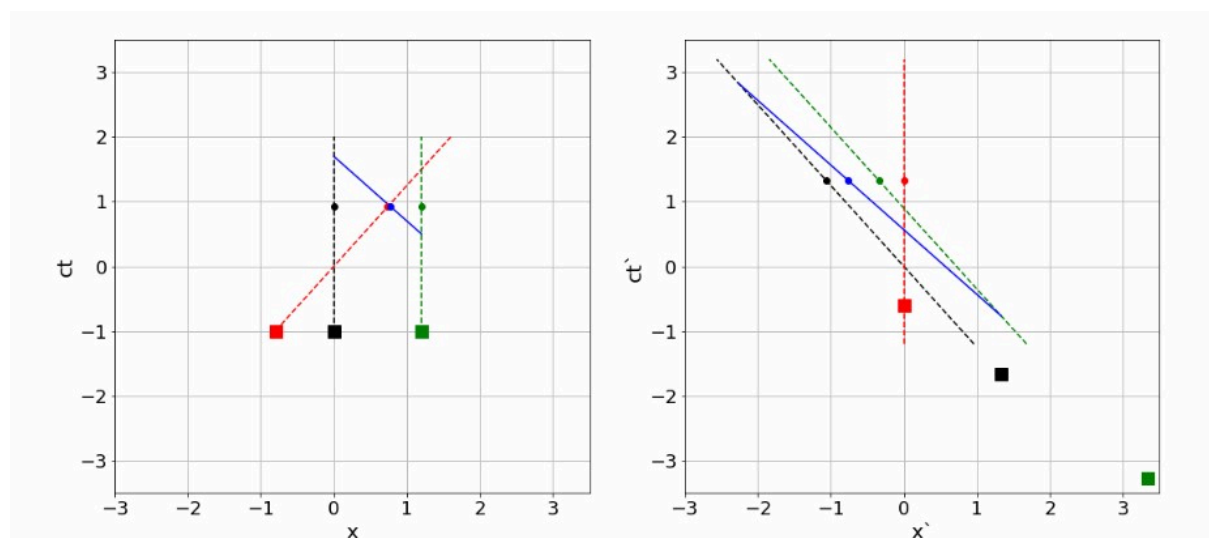
Figure 3.200: An animation of events as seen by different observers.
