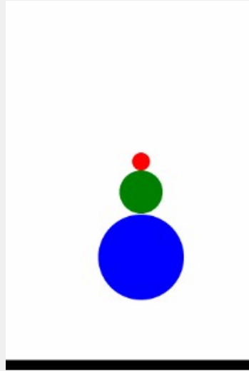
Figure 2.113: Bouncing of three (super)balls.
