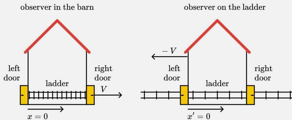
Figure 3.203: Ladder & Barn: perspective from two observers.
