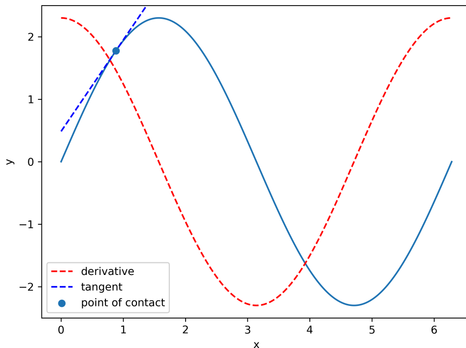
Figure 4.239: A sine function with both its derivative (a cosine function) and its tangent at a certain point.
