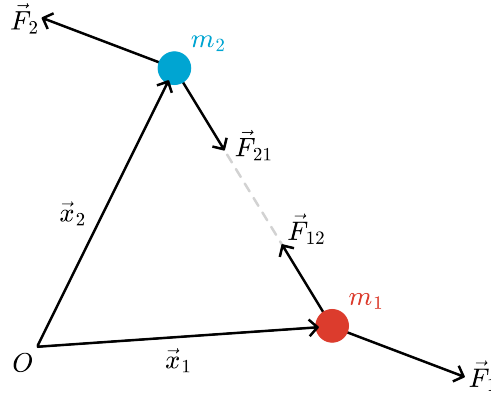
Figure 2.170: Two-particle system, with an action/reaction pair of forces.
