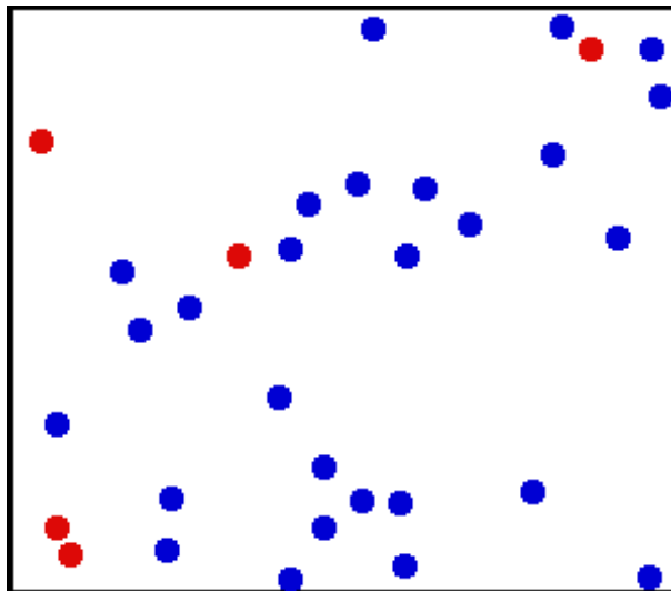
Figure 2.164: Computing multiple collisions by hand is quite challenging, but can be done ‘easily’ with the computer. Figure made by A. Greg , public domain
