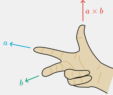
Figure 2.71: Right hand rule for cross products. Adapted from Wikimedia Commons , licensed under CC-BY-SA 4.0.
