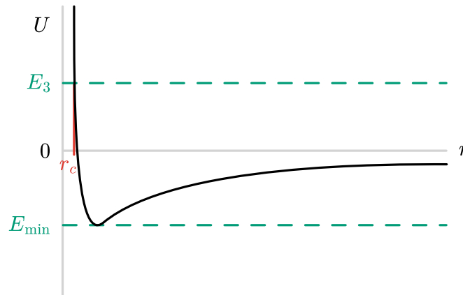
Figure 2.88: Total energy larger than 0.
