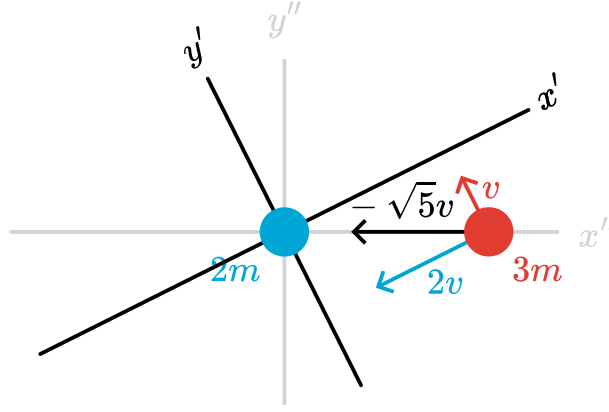
Figure 2.160: Rotating the coordinate system.
