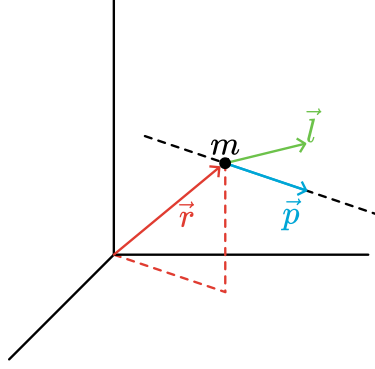
Figure 2.74: Angular momentum of a free particle.
