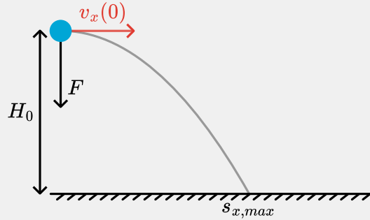
Figure 2.21: A sketch of the situation where an object is thrown horizontally and the horizontal distance should be calculated.
