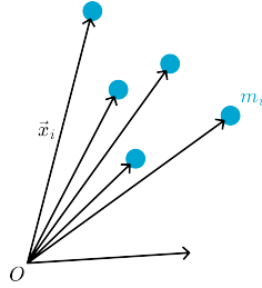
Figure 2.181: Many particle system.
