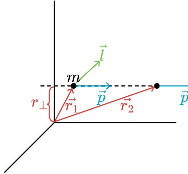
Figure 2.75: Angular momentum of a free particle is constant.
