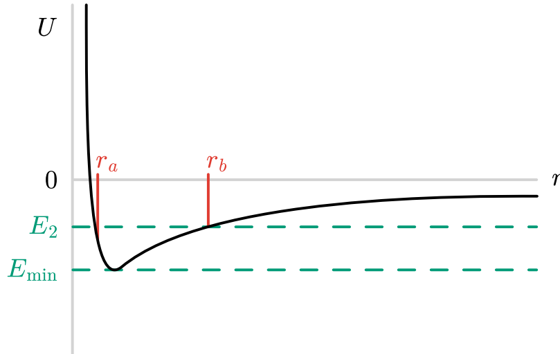
Figure 2.87: Total energy between 0 and minimum of effective potential.
