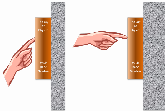
Figure 2.25: A book is held in place against a wall. The magnitude of the force applied by the hand on the book is the same in the left and the right scenarios.
