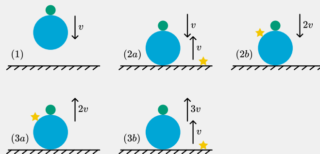
Figure 2.112: Bouncing balls.
