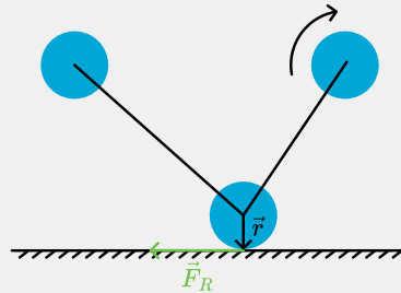
Figure 2.76: A bouncing basketball.
