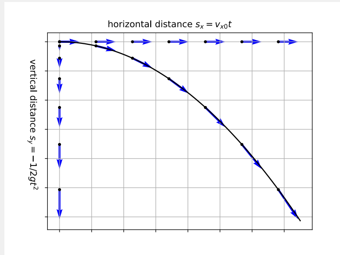
Figure 2.22: The parabolic motion is visualized with blue velocity vectors v , v_x and v_y shown at various points along the trajectory for a constant time interval.
