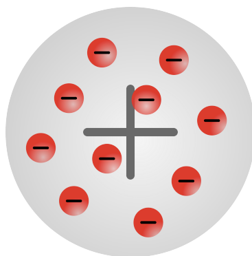
Figure 3.187: Plum pudding model according to Joseph Thomson. From Wikimedia Commons , public domain.
