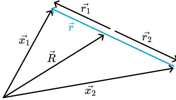
Figure 2.162: Center of mass.
