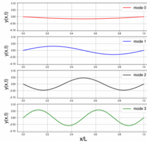
Figure 2.145: Standing waves in a string.
