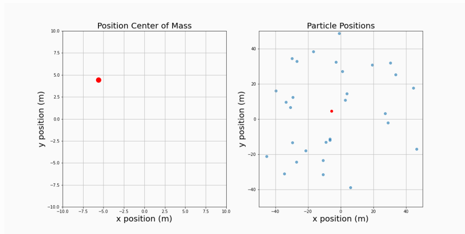
Figure 2.185: 30 particles: left motion of the center of mass, right motion of all particles.
