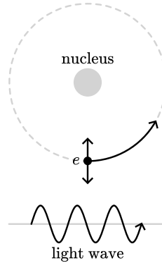
Figure 2.142: Simple model of electron-light scattering.
