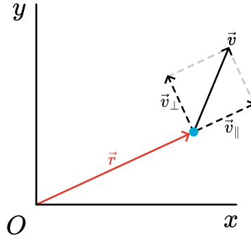
Figure 2.85: The coordinate r is the distance from the sun to the earth. Its time derivative ( \dot{r} = \frac{dr}{dt} = v_{//} ) is the velocity of the earth away from the sun.
