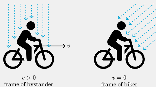
Figure 2.115: Riding a bike in the rain.
