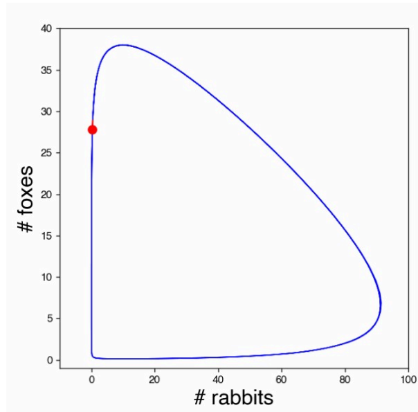
Figure 2.125: Phase plot of the rabbit-fox prey-predator model. The red dot shows the population at different times. Note that the number of rabbits quickly increases when there are very few foxes. However, at some point the number of foxes also goes up and soon the start reducing the rabbits, while increasing in numbers themselves. That is not sustainable and when the number of rabbits is brought down substantially, also the number of foxes decreases, until both are almost extinct and the cycle repeats.
