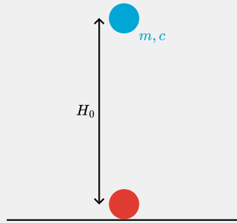
Figure 2.165: The iron ball with mass m is dropped from a height H_0 . What will the temperature increase be?
