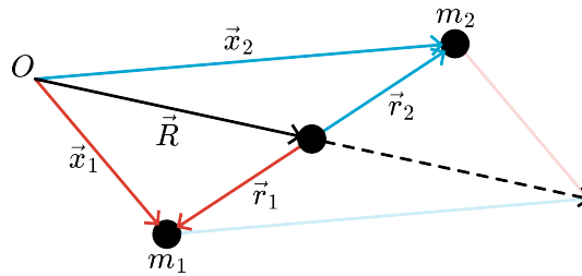
Figure 2.171: Center of Mass and relative coordinates.
