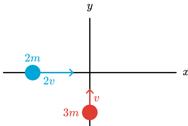
Figure 2.158: Example of a 2D elastic collision.
