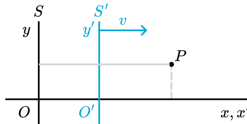
Figure 2.110: Two inertial observers S and S' and their coordinate systems.
