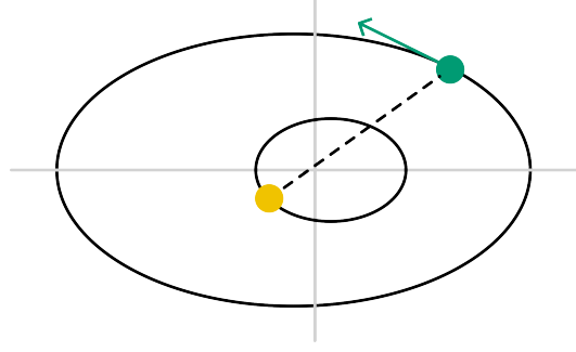
Figure 2.172: Kepler revisited.
