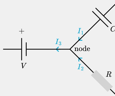
Figure 2.133: Currents in and out of a node must add to zero.
