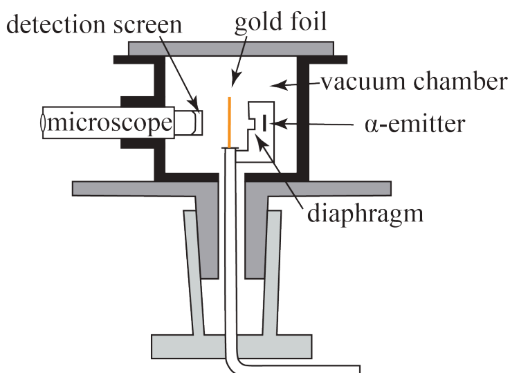
Figure 3.188: Experimental setup of \alpha -scattering at a gold foil.
