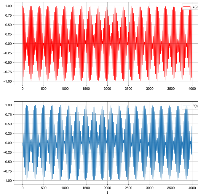
Figure 2.128: Numerical solution of the Wilberforce pendulum using a higher-order numerical method.
