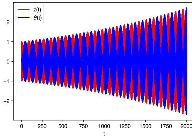
Figure 2.127: Numerical solution of the Wilberforce pendulum using a (too) simple numerical method.
