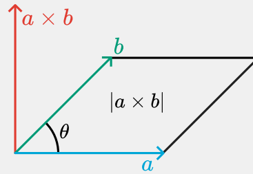
Figure 2.72: Area of cross products. From Wikimedia Commons , public domain.
