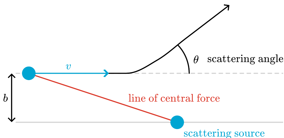
Figure 3.192: Scattering of an incoming particle at a fixed source.
