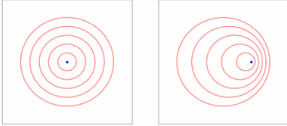
Figure 3.208: Effect on sound waves due to motion.
