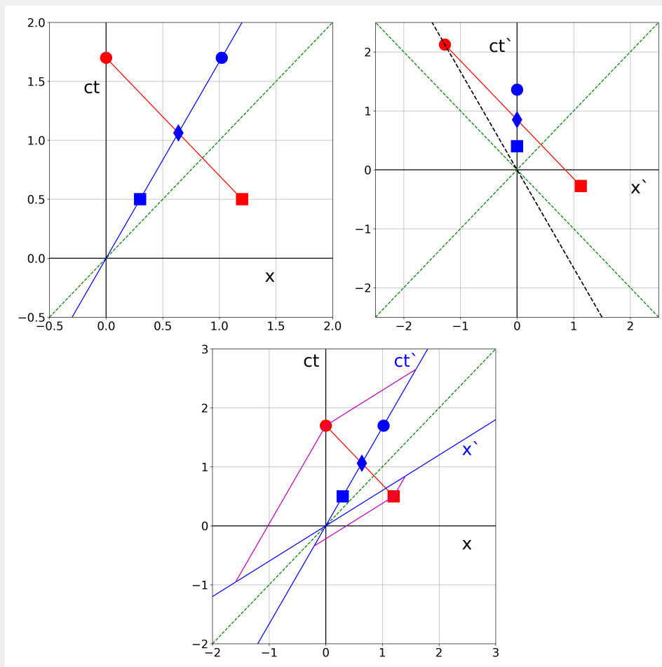
Figure 3.233: top left: S , top right: S' , bottom: Minkowski diagram.
