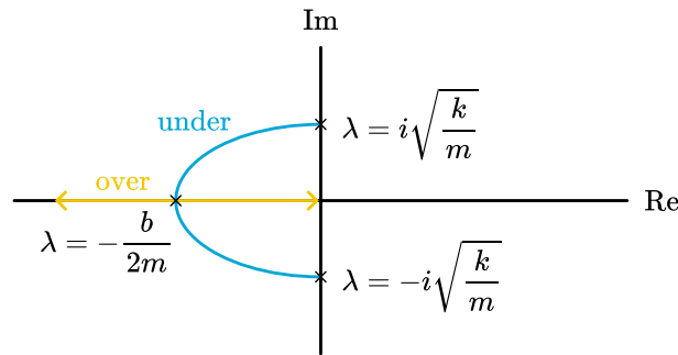
Figure 2.140: Evolution of \lambda as a function of b in the complex plane.
