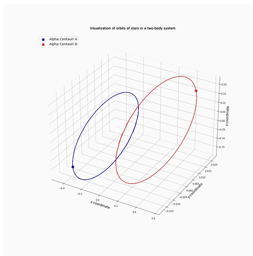
Figure 2.178: Alpha Centauri A and B circling each other.
