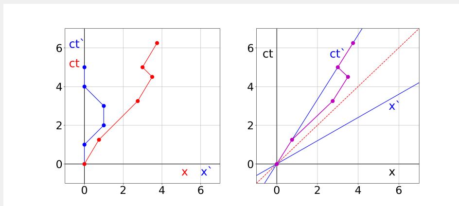
Figure 3.232: left: S and S' in the same diagram; right: Minkowski diagram.
