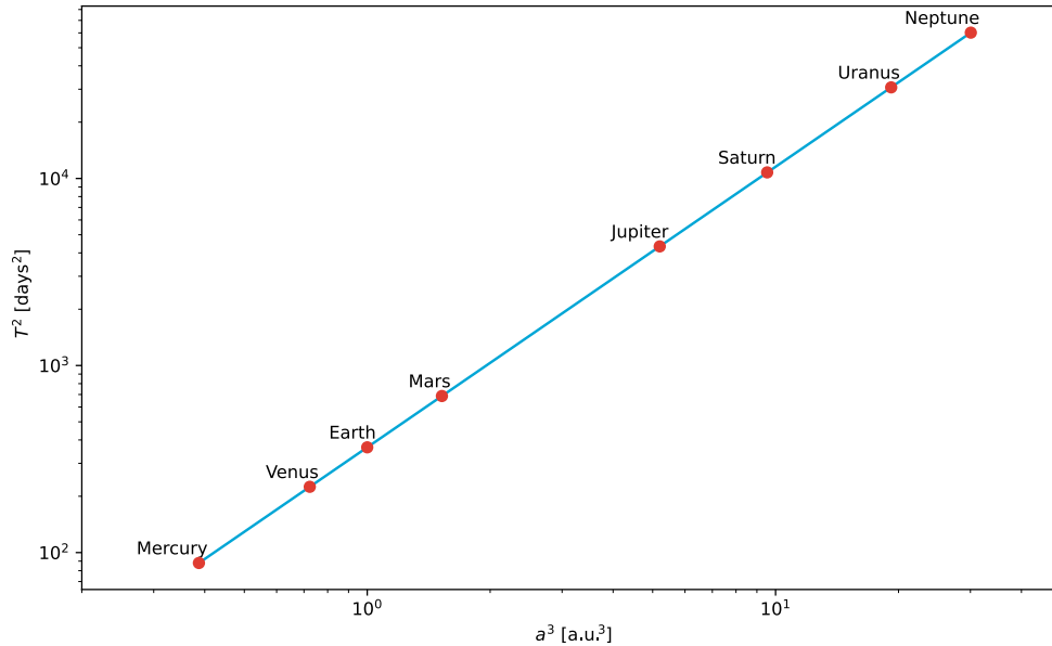
Figure 2.91: Kepler 3 for our solar system.
