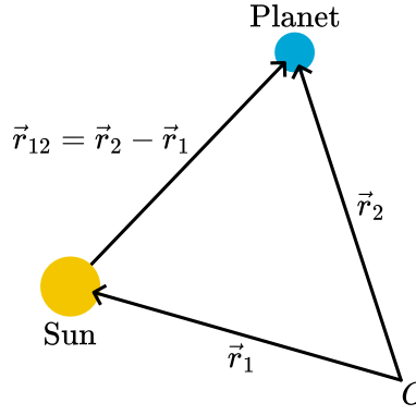
Figure 2.83: The sun and a planet.
