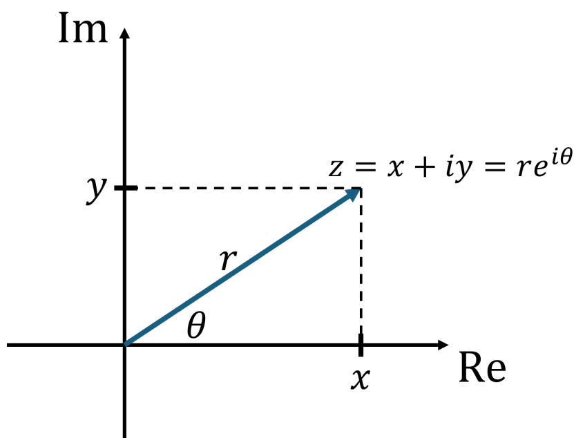
Figure 4.240: The complex plane, where the horizontal axis represents the real part and the vertical axis represents the imaginary part of a complex number.
