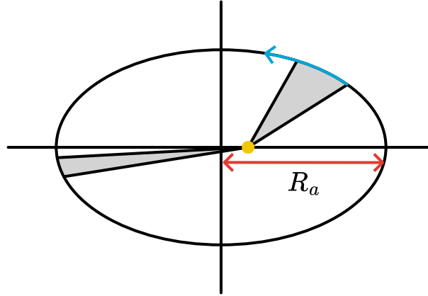
Figure 2.82: Kepler's 2nd Law of Equal Area.
