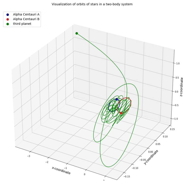
Figure 2.180: Alpha Centauri A and B circling each other with a third object. The third ‘planet’ is finally escaping into space. Note: this is a chaotic system and computations need great care.
