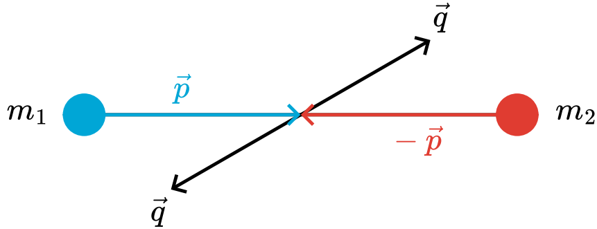
Figure 2.163: Collision in center of mass frame.
