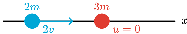
Figure 2.156: Example of a 1D elastic collision.
