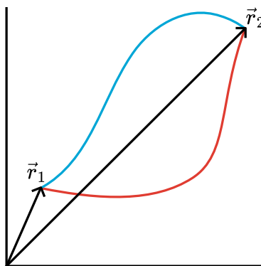
Figure 2.53: Two different paths. In a conservative force field the work done will be the same.
