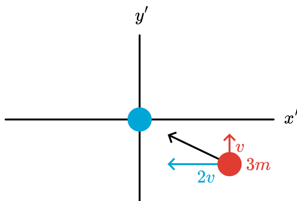
Figure 2.159: Applying the Galilean Transformation.
