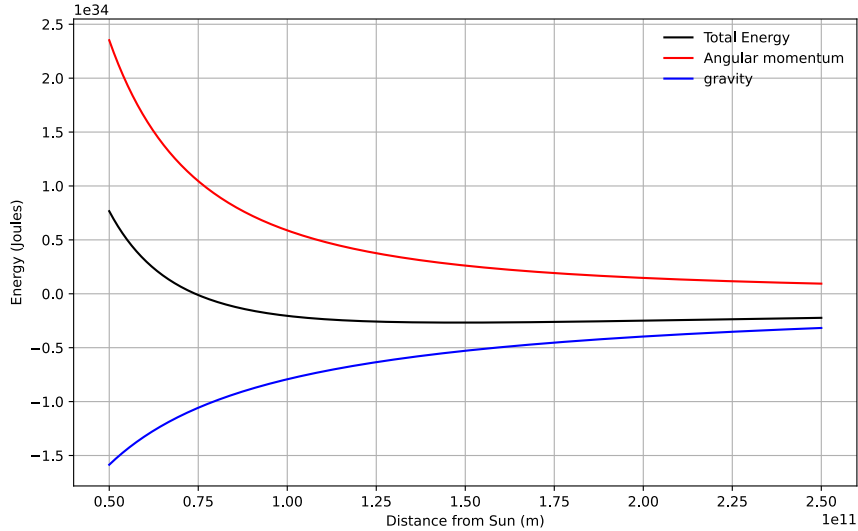
Figure 2.86: Energies related to our planet, with a minimum around 1.5e11m .
