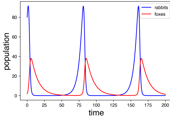
Figure 2.124: Periodic time evolution of the population of rabbits and foxes.
