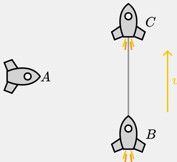
Figure 3.205: Bell's paradox: accelerating spaceships and a thin wire.
