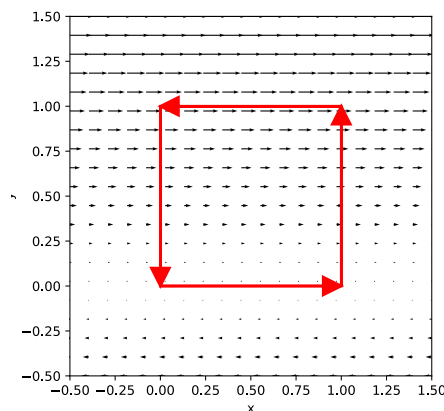
Figure 2.60: The force field that the professor is cycling in.
