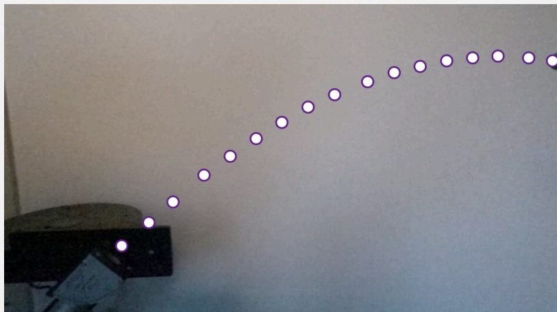
Figure 2.23: A parabolic motion visualized, with the position stored per time unit
