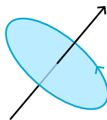
Figure 2.69: The rotation is given by the black arrow. You can find it by using the corkscrew rule: rotating a corkscrew as the blue arrow indicates gives that the screw moves forward like the black arrow.
