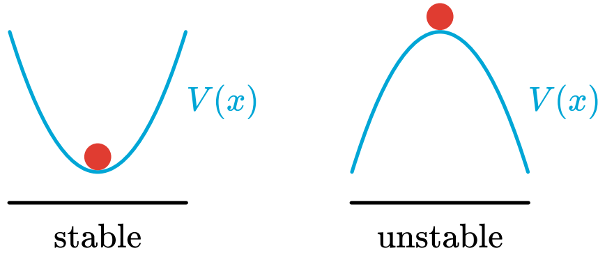
Figure 2.57: Stable and unstable position of a particle in a potential.
