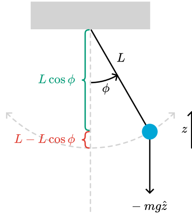
Figure 2.137: Potential energy of a pendulum.
