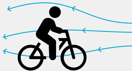
Figure 2.114: Air resistance on cyclist.
