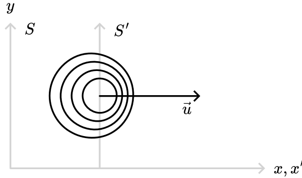
Figure 3.209: Observer S' and source both moving with respect to S .
