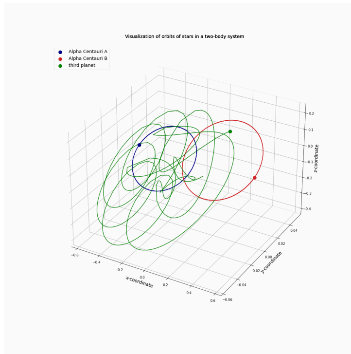
Figure 2.179: Alpha Centauri A and B circling each other with a third object.
