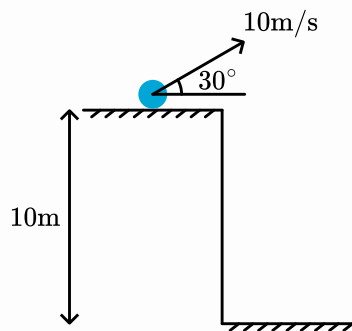
Figure 2.34: A ball on a hill launched under an angle.
