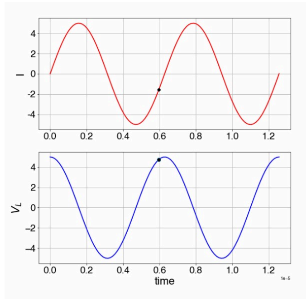
Figure 2.135: Harmonic oscillation of an LC-circuit.
