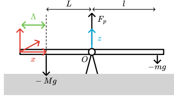
Figure 2.68: Free-body diagram with the origin located at the seesaw's end.
